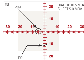
MOVE YOUR RETICLE SO THAT IT INTERSECTS BOTH YOUR POA AND POI, AS SHOWN ABOVE. NOTE THE OFFSETS TO BOTH WINDAGE AND ELEVATION
