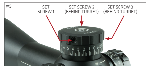
#5 TURRET SET SCREWS [3x PER TURRET]
