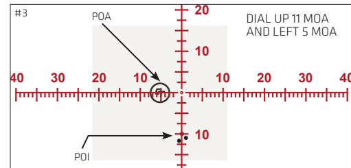
#3 MOVE YOUR RETICLE SO THAT IT INTERSECTS BOTH YOUR POA AND POI, AS SHOWN ABOVE. NOTE THE OFFSETS TO BOTH WINDAGE AND ELEVATION
