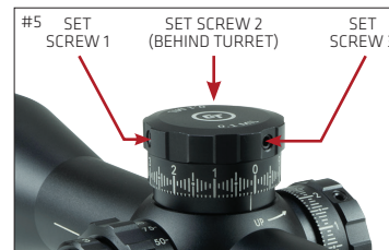
TURRET SET SCREWS [3x PER TURRET]
